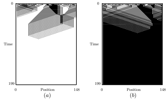
Figure 3: These are examples of majority problem classification by the rule found by David, Forrest and Koza. Both are correct classifications (a) with 74 ones in the initial state, (b) with 75.
