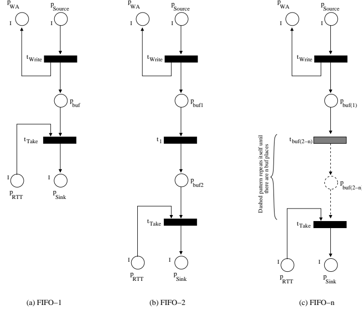
Fig. 6. The FIFO 1, 2 and n Channel EN Systems
