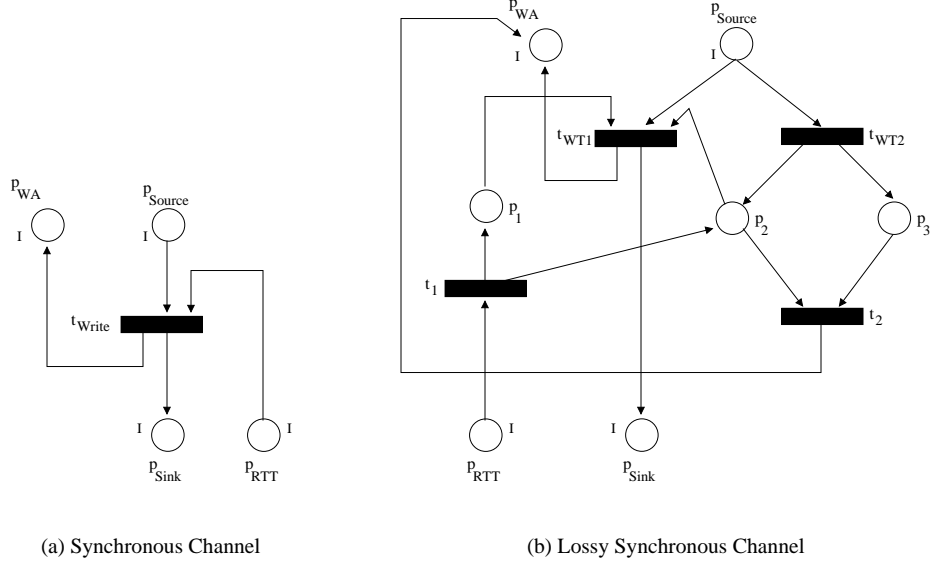
Fig. 5. The Synchronous and Lossy Synchronous Channel EN Systems
