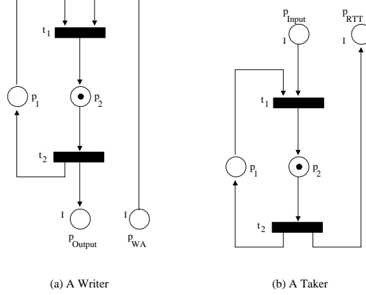
Fig. 3. A Writer and a Taker EN System
