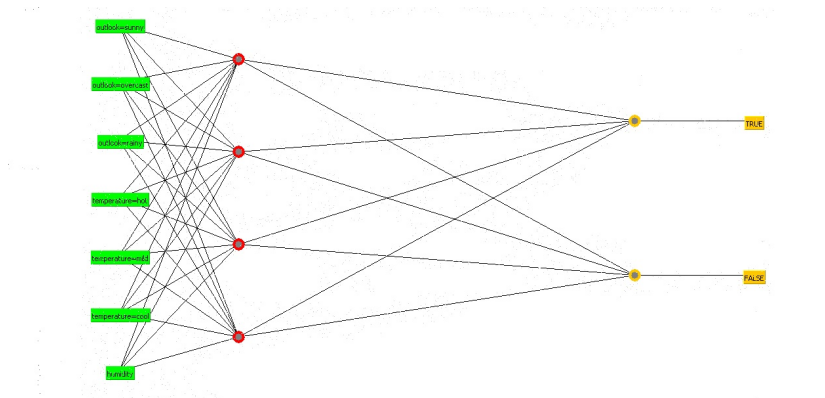
Figure 7: Example of a neural network (Weka, weather data set)
