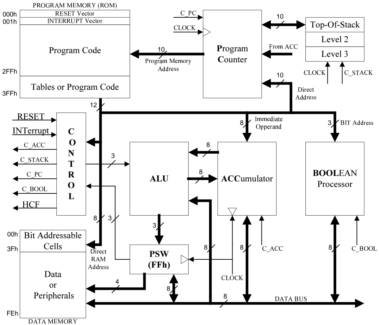
Fig.2. Ims8NI core - Block diagram
