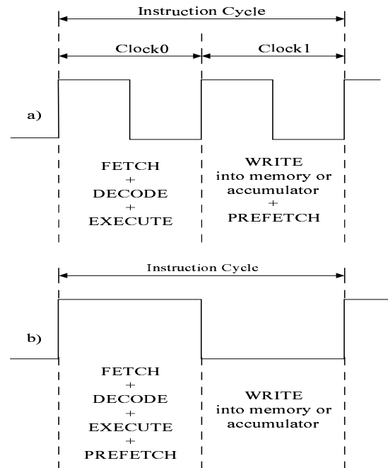
Fig.4. Two possible timing diagrams of Ims8NI
